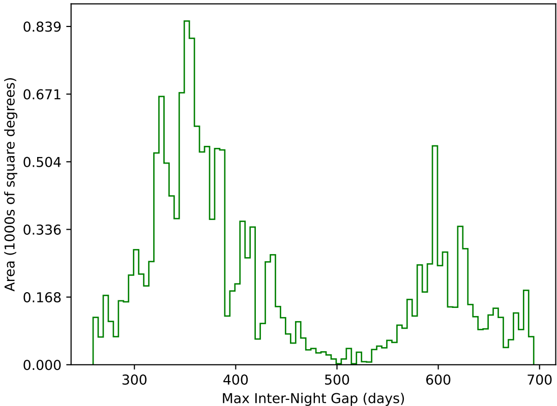
too_elab_r128_d2_gz_v3.4_10yrs WFD g band: Max Inter-Night Gap
