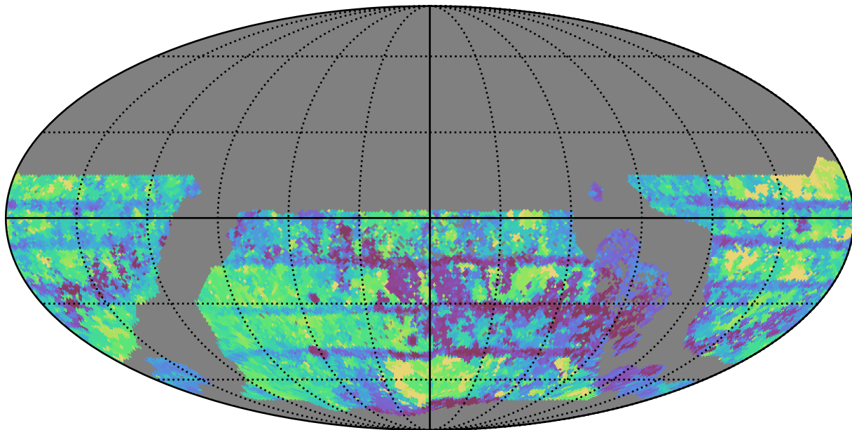
too_elab_r128_d2_gz_v3.4_10yrs WFD all bands: Max Inter-Night Gap
