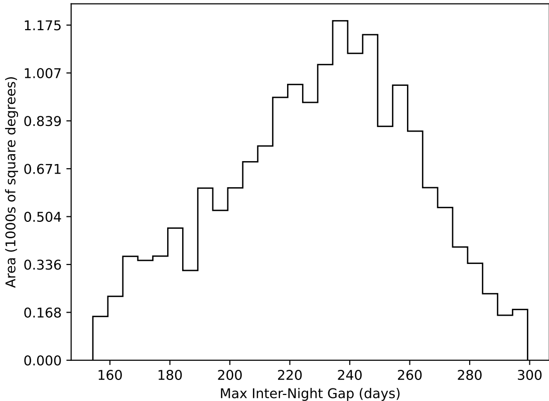
too_elab_r128_d2_gz_v3.4_10yrs WFD all bands: Max Inter-Night Gap
