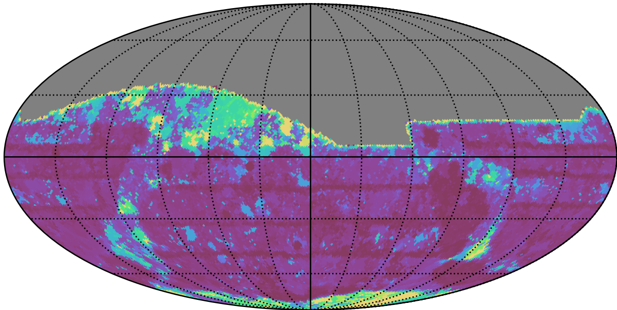
too_elab_r128_d2_gz_v3.4_10yrs All sky z band: Max Inter-Night Gap
