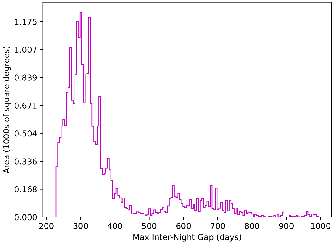
too_elab_r128_d2_gz_v3.4_10yrs All sky z band: Max Inter-Night Gap
