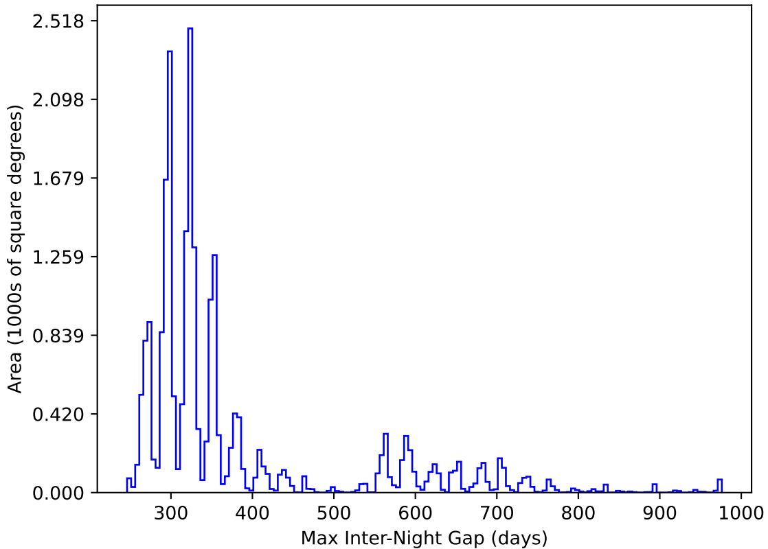
too_elab_r128_d2_gz_v3.4_10yrs All sky y band: Max Inter-Night Gap
