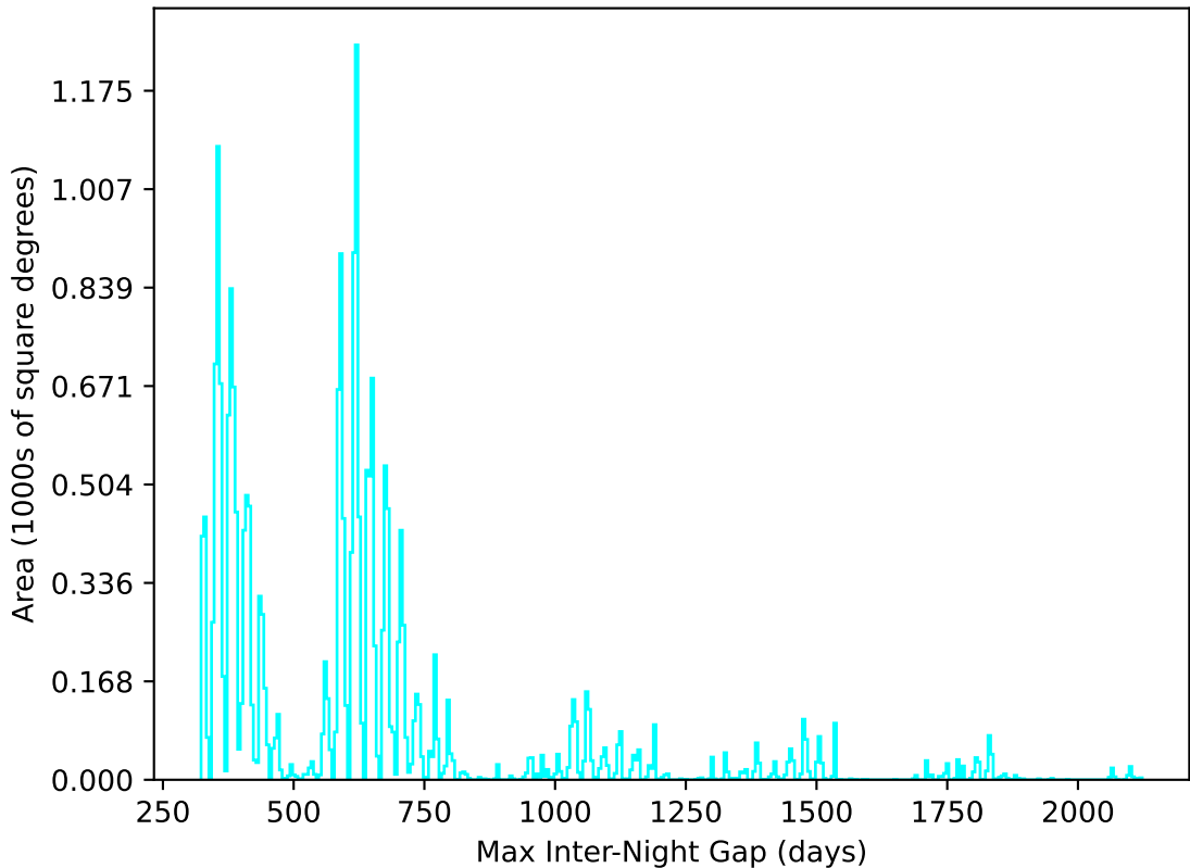
too_elab_r128_d2_gz_v3.4_10yrs All sky u band: Max Inter-Night Gap
