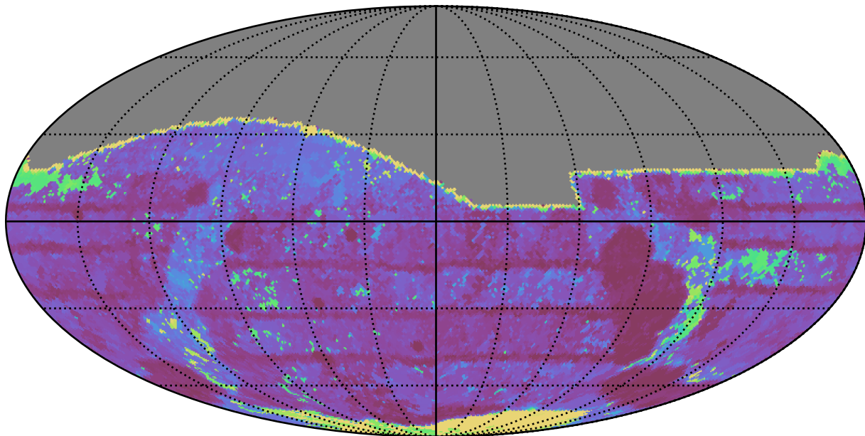
too_elab_r128_d2_gz_v3.4_10yrs All sky r band: Max Inter-Night Gap
