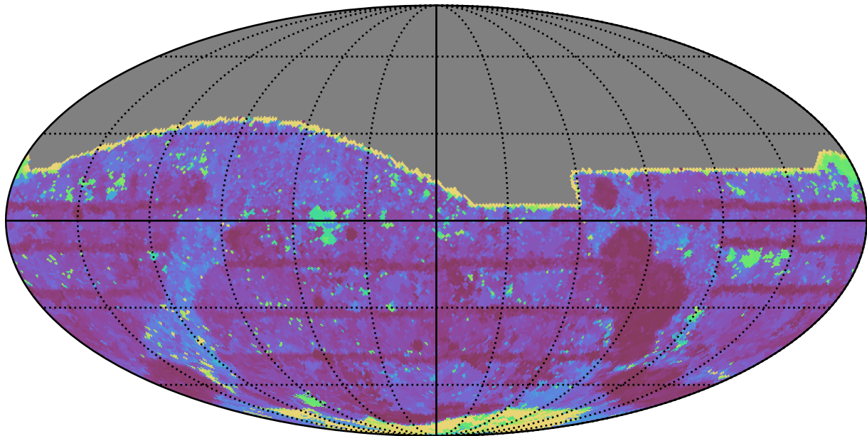
too_elab_r128_d2_gz_v3.4_10yrs All sky i band: Max Inter-Night Gap
