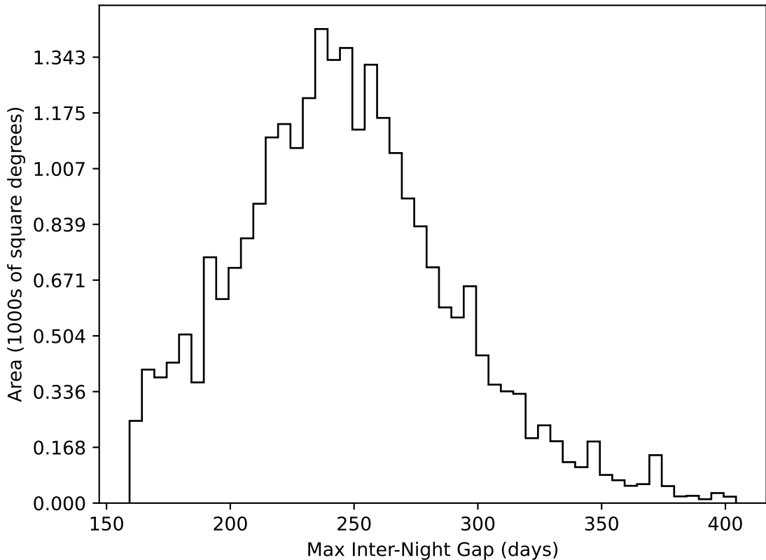
too_elab_r128_d2_gz_v3.4_10yrs All sky all bands: Max Inter-Night Gap
