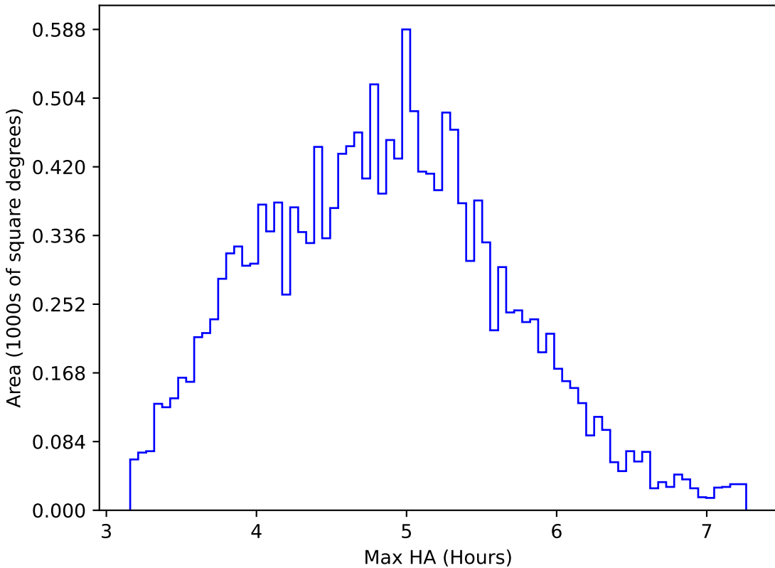
too_elab_r128_d2_gz_v3.4_10yrs WFD z band: Max HA
