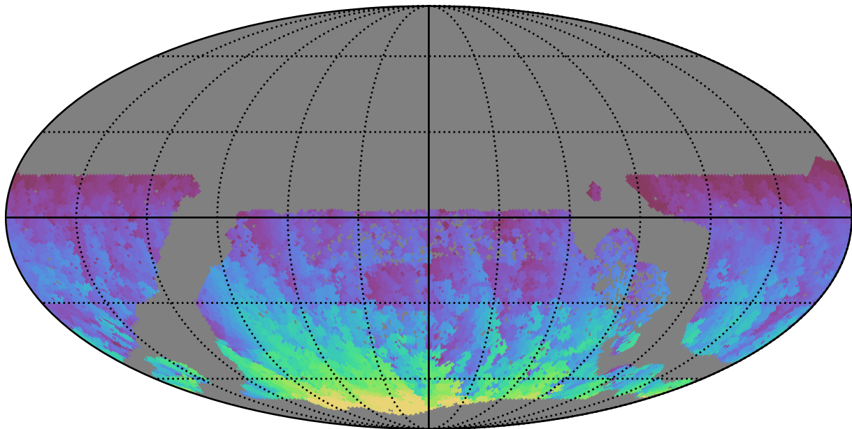
too_elab_r128_d2_gz_v3.4_10yrs WFD y band: Max HA
