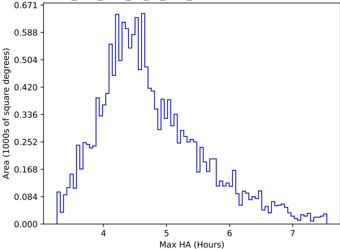
too_elab_r128_d2_gz_v3.4_10yrs WFD y band: Max HA
