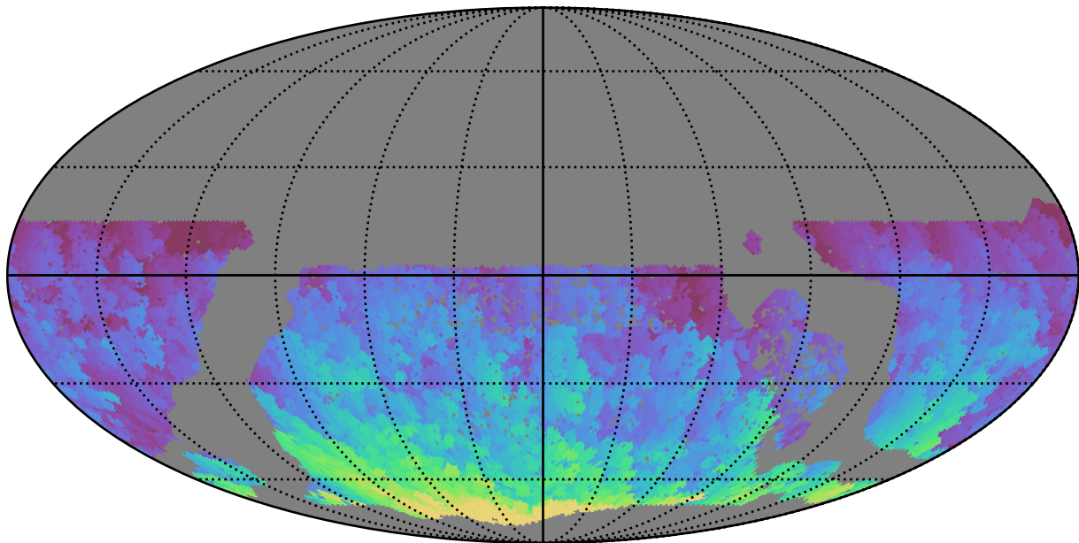
too_elab_r128_d2_gz_v3.4_10yrs WFD r band: Max HA
