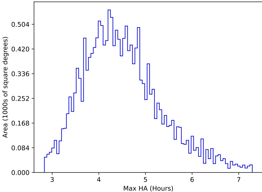
too_elab_r128_d2_gz_v3.4_10yrs WFD r band: Max HA
