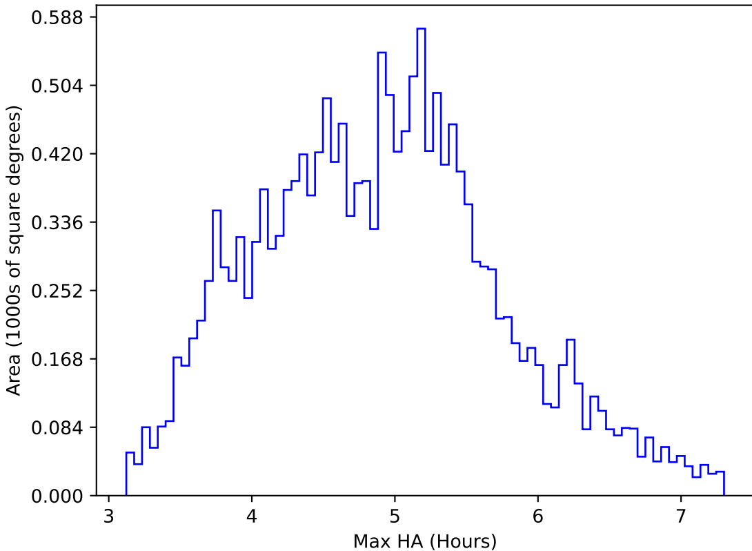
too_elab_r128_d2_gz_v3.4_10yrs WFD i band: Max HA
