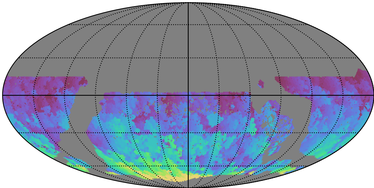
too_elab_r128_d2_gz_v3.4_10yrs WFD g band: Max HA
