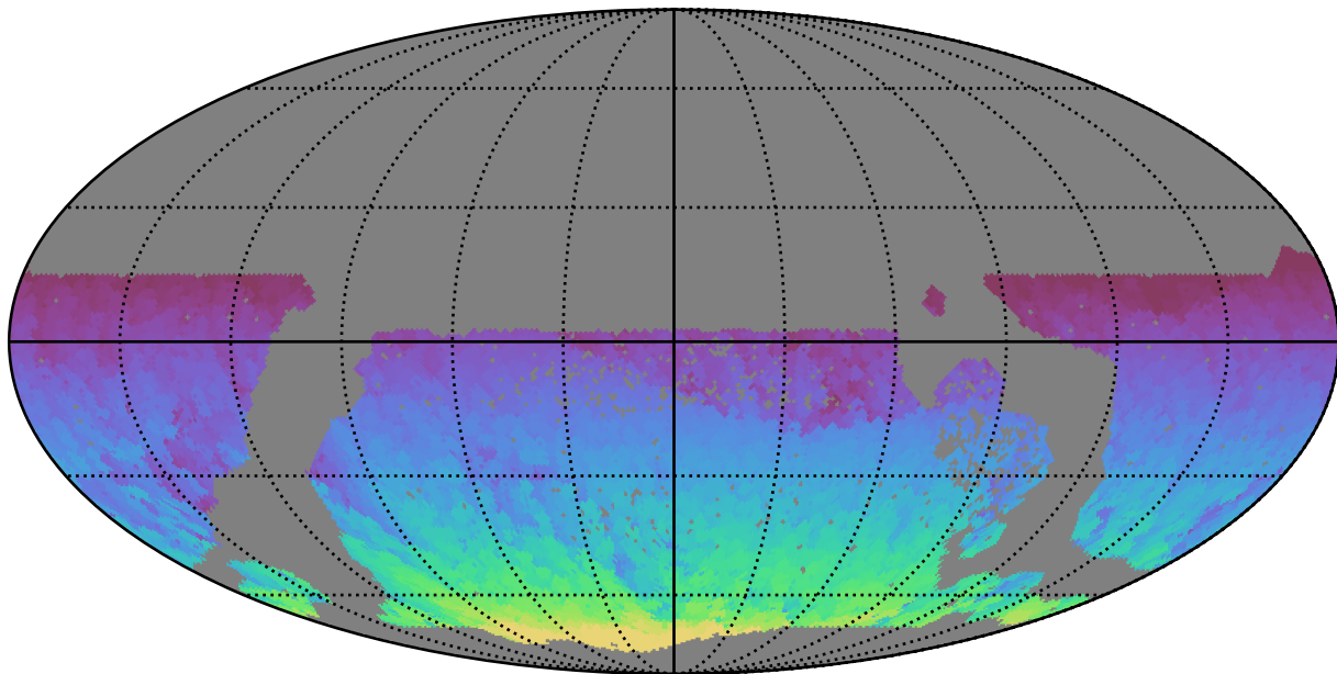
too_elab_r128_d2_gz_v3.4_10yrs WFD all bands: Max HA
