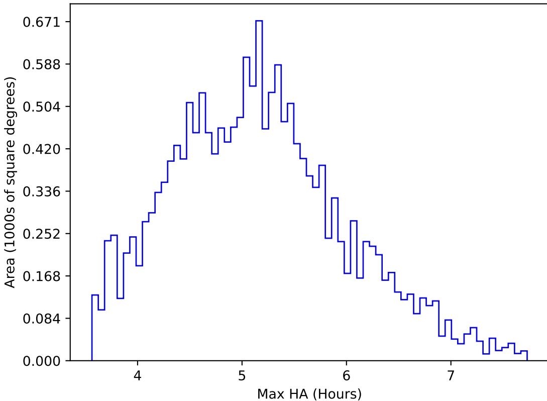
too_elab_r128_d2_gz_v3.4_10yrs WFD all bands: Max HA
