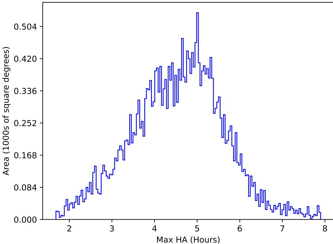
too_elab_r128_d2_gz_v3.4_10yrs All sky z band: Max HA
