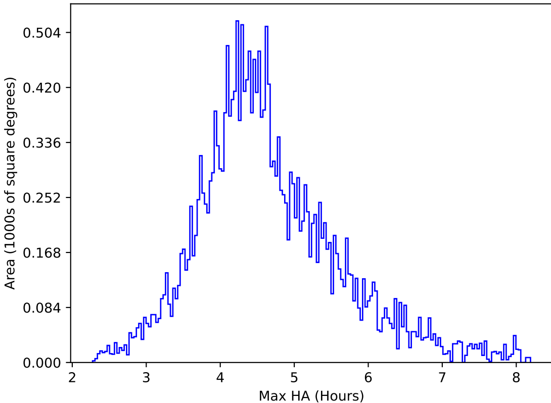
too_elab_r128_d2_gz_v3.4_10yrs All sky y band: Max HA
