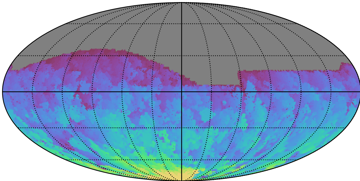
too_elab_r128_d2_gz_v3.4_10yrs All sky g band: Max HA
