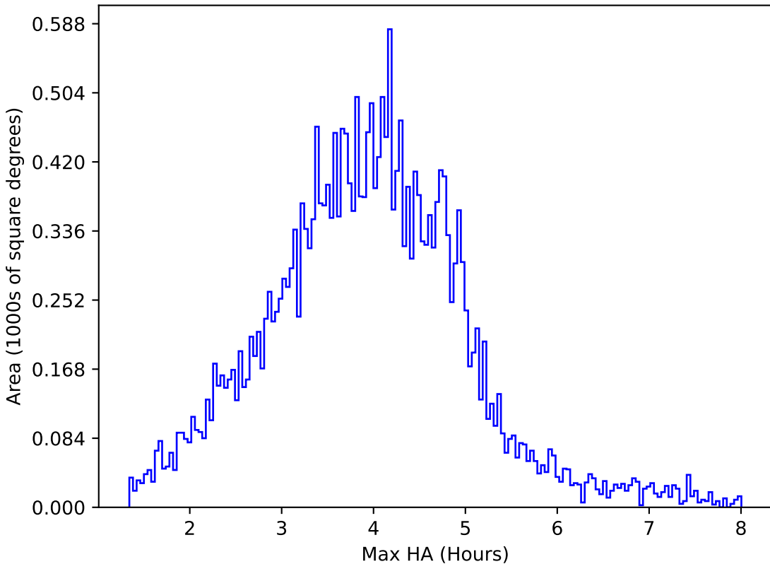
too_elab_r128_d2_gz_v3.4_10yrs All sky g band: Max HA
