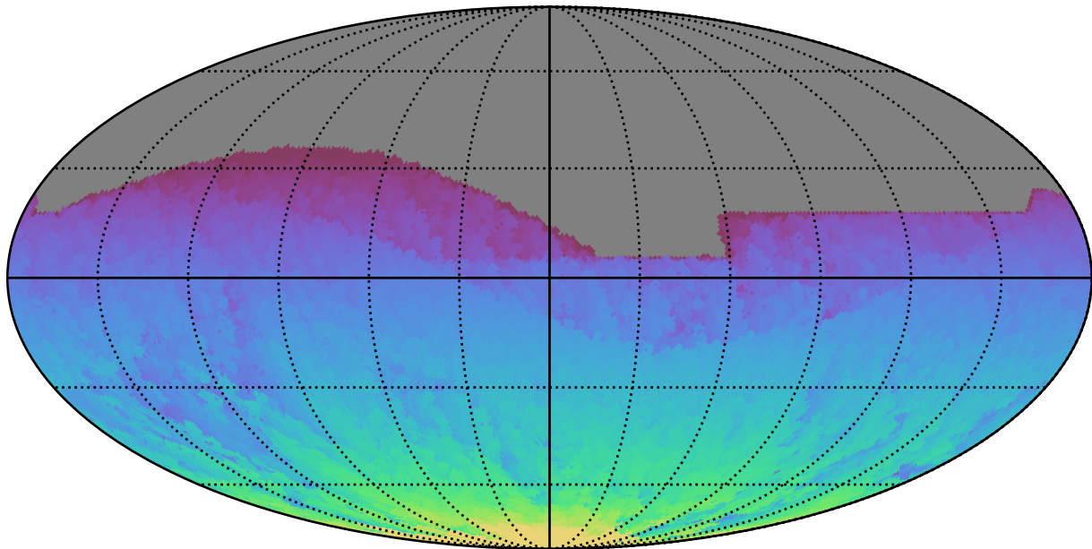
too_elab_r128_d2_gz_v3.4_10yrs All sky all bands: Max HA
