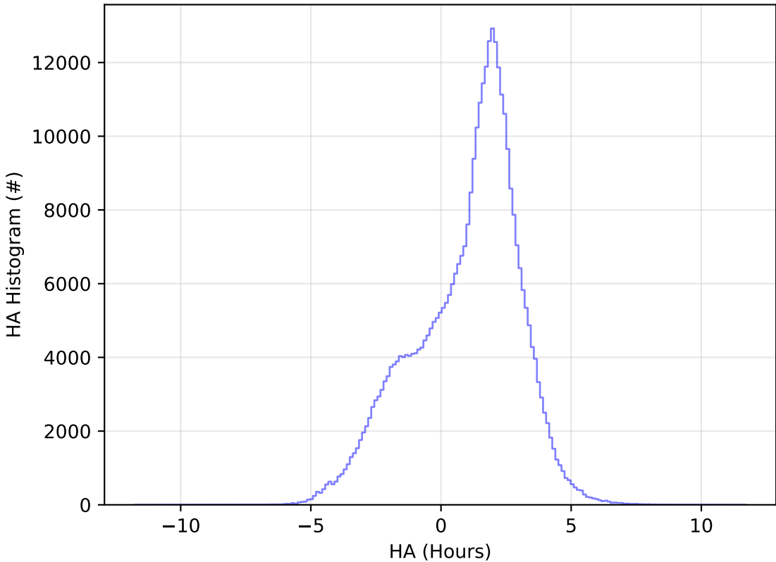
too_elab_r128_d2_gz_v3.4_10yrs WFD y band: HA Histogram
