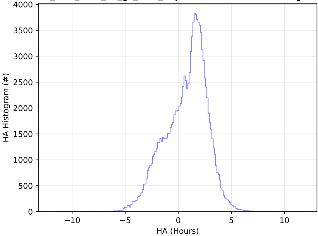
too_elab_r128_d2_gz_v3.4_10yrs WFD u band: HA Histogram
