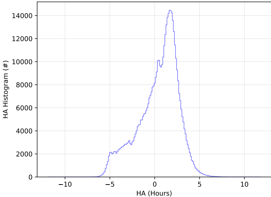
too_elab_r128_d2_gz_v3.4_10yrs WFD r band: HA Histogram
