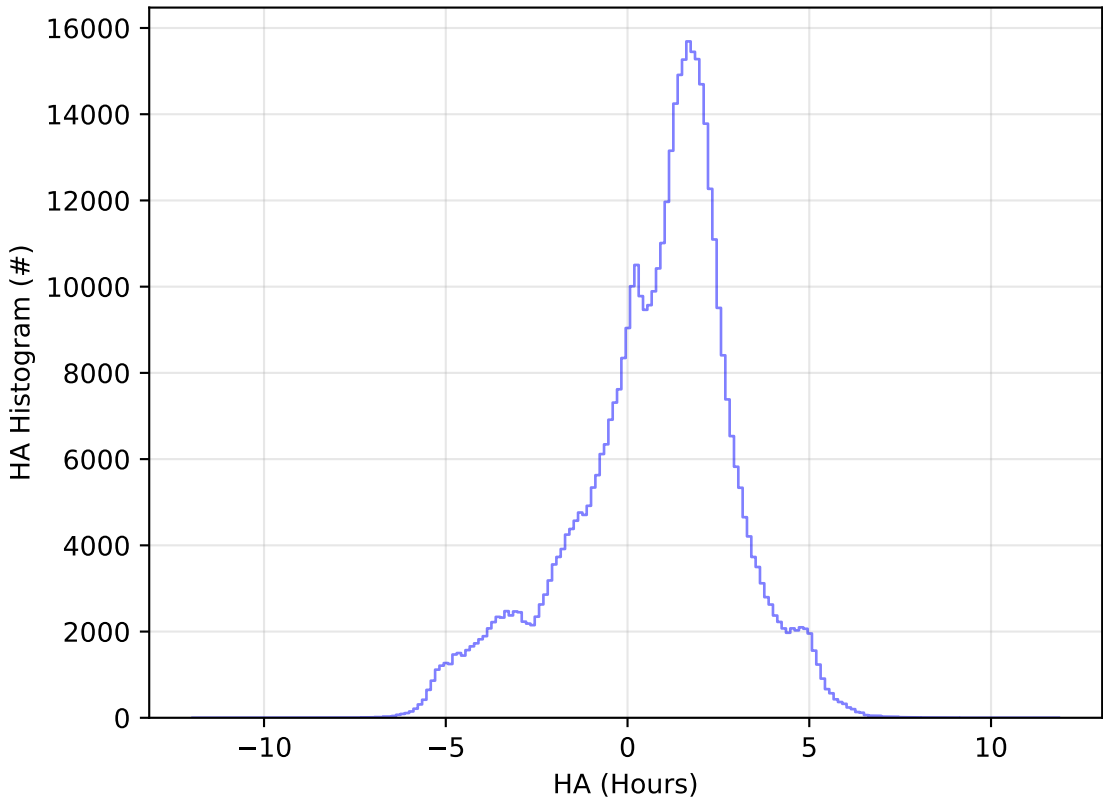
too_elab_r128_d2_gz_v3.4_10yrs WFD i band: HA Histogram
