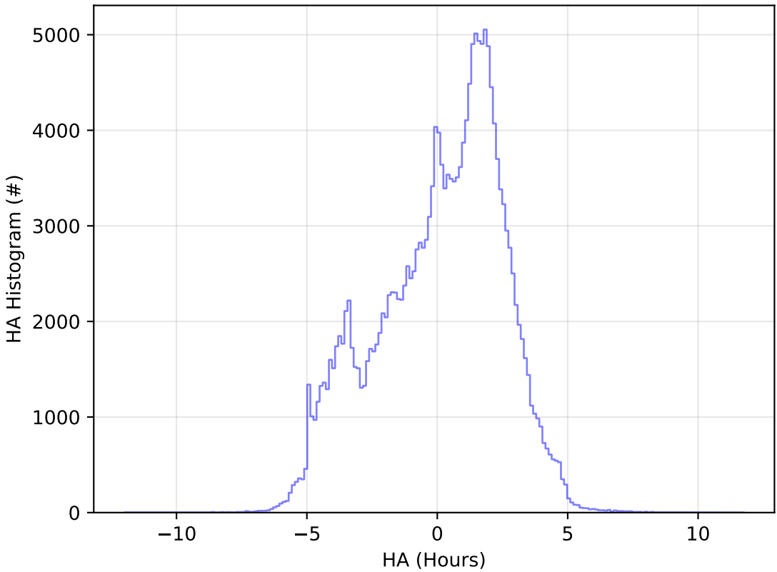
too_elab_r128_d2_gz_v3.4_10yrs WFD g band: HA Histogram
