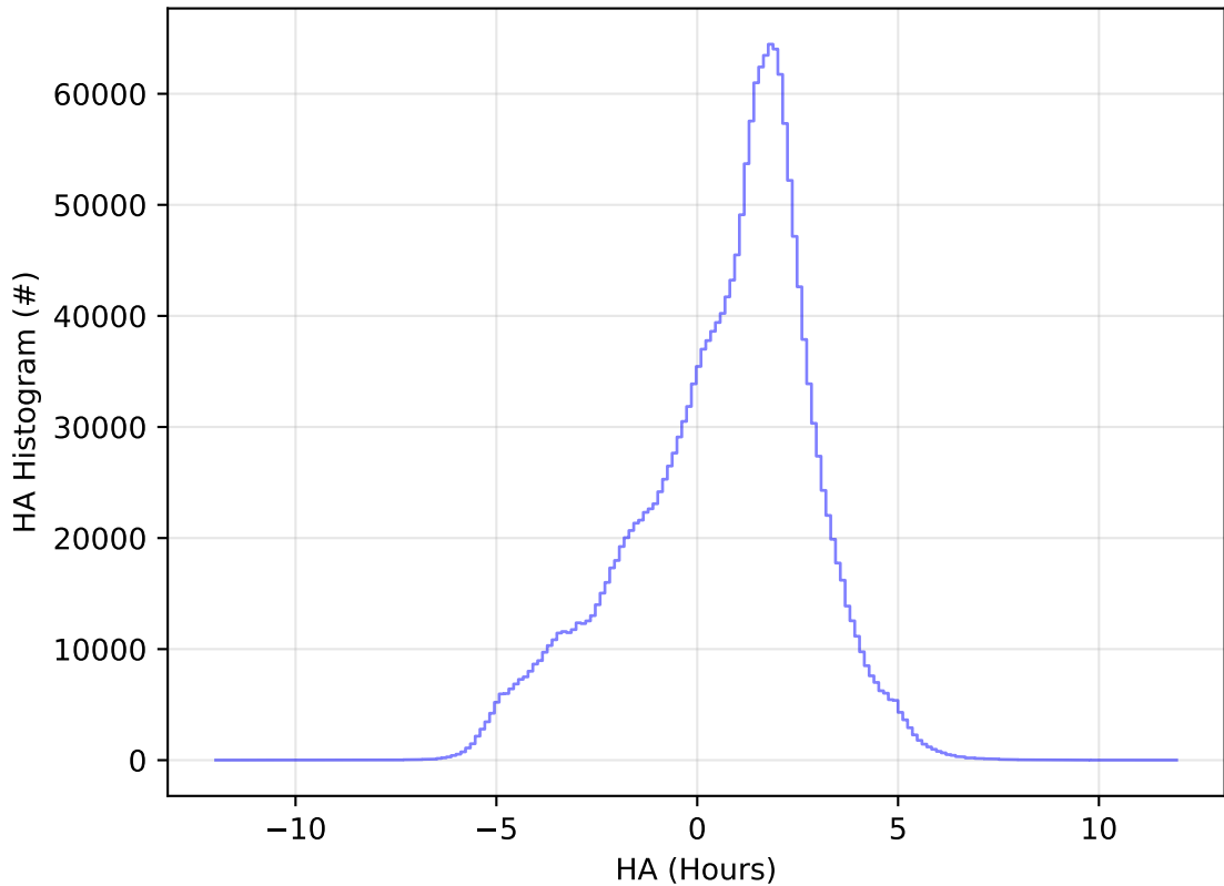
too_elab_r128_d2_gz_v3.4_10yrs WFD all bands: HA Histogram
