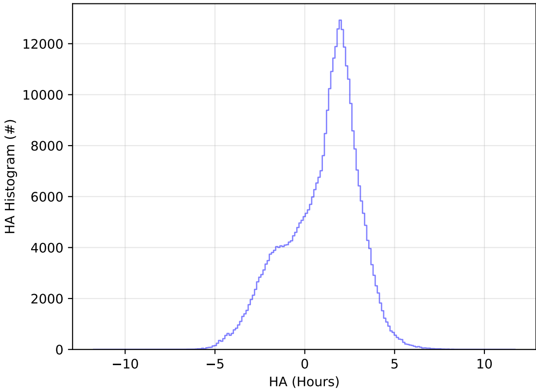
too_elab_r128_d2_gz_v3.4_10yrs All sky y band: HA Histogram
