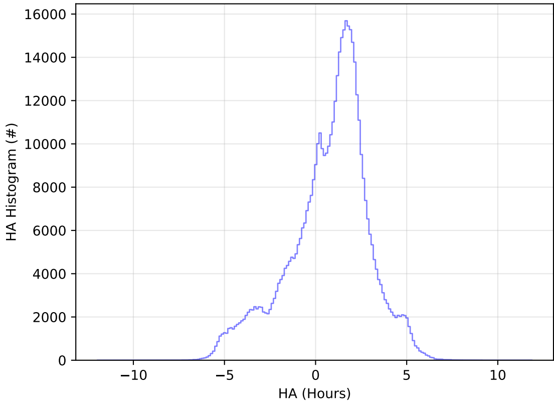
too_elab_r128_d2_gz_v3.4_10yrs All sky i band: HA Histogram
