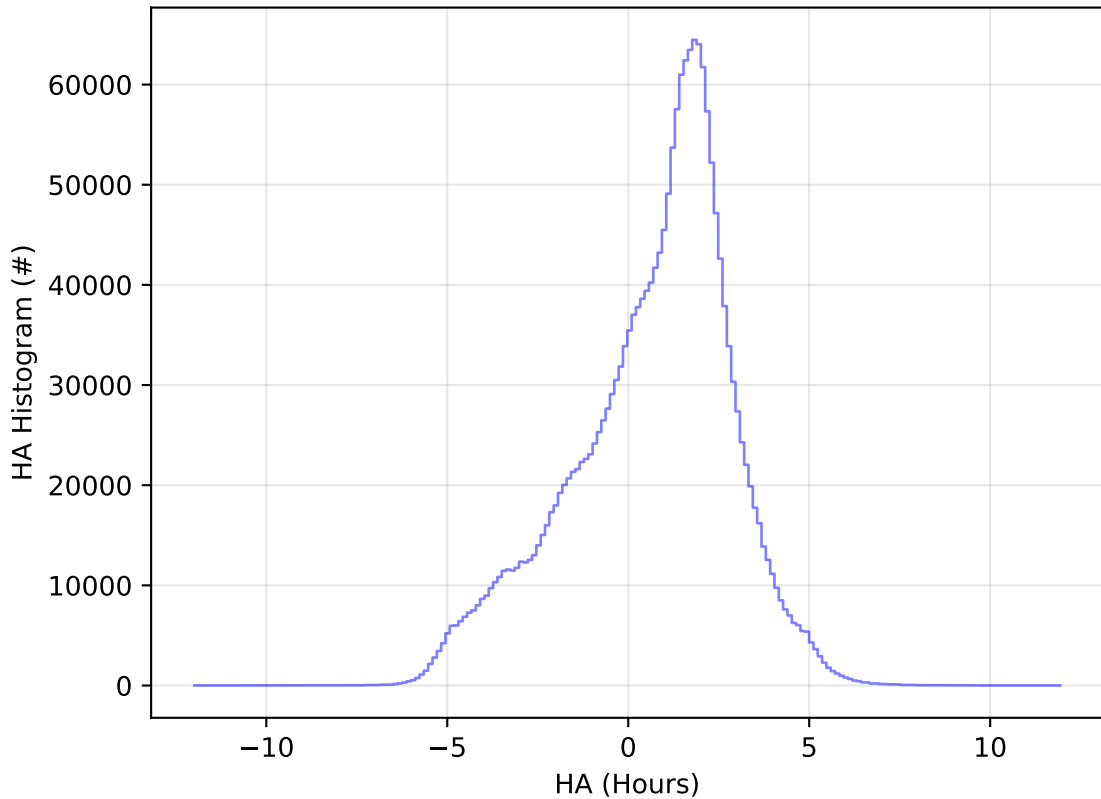
too_elab_r128_d2_gz_v3.4_10yrs All sky all bands: HA Histogram
