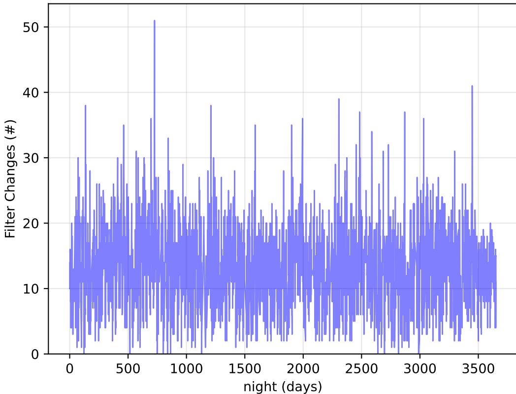
too_elab_r128_d2_gz_v3.4_10yrs Per Night: Filter Changes
