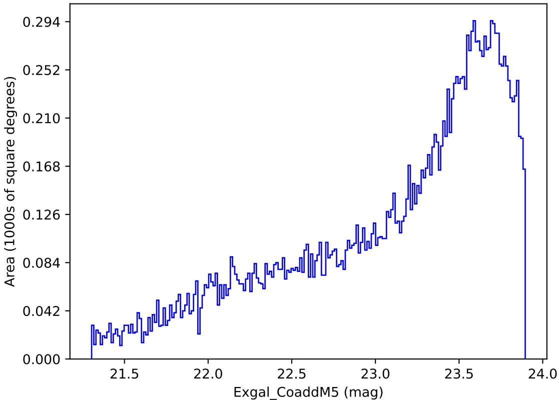
too_elab_r128_d2_gz_v3.4_10yrs Yr 3-4 y band: Exgal_CoaddM5
