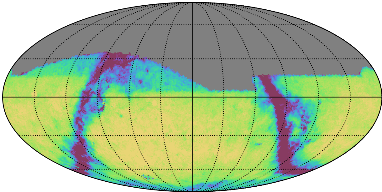
too_elab_r128_d2_gz_v3.4_10yrs Yr 1 r band: Exgal_CoaddM5
