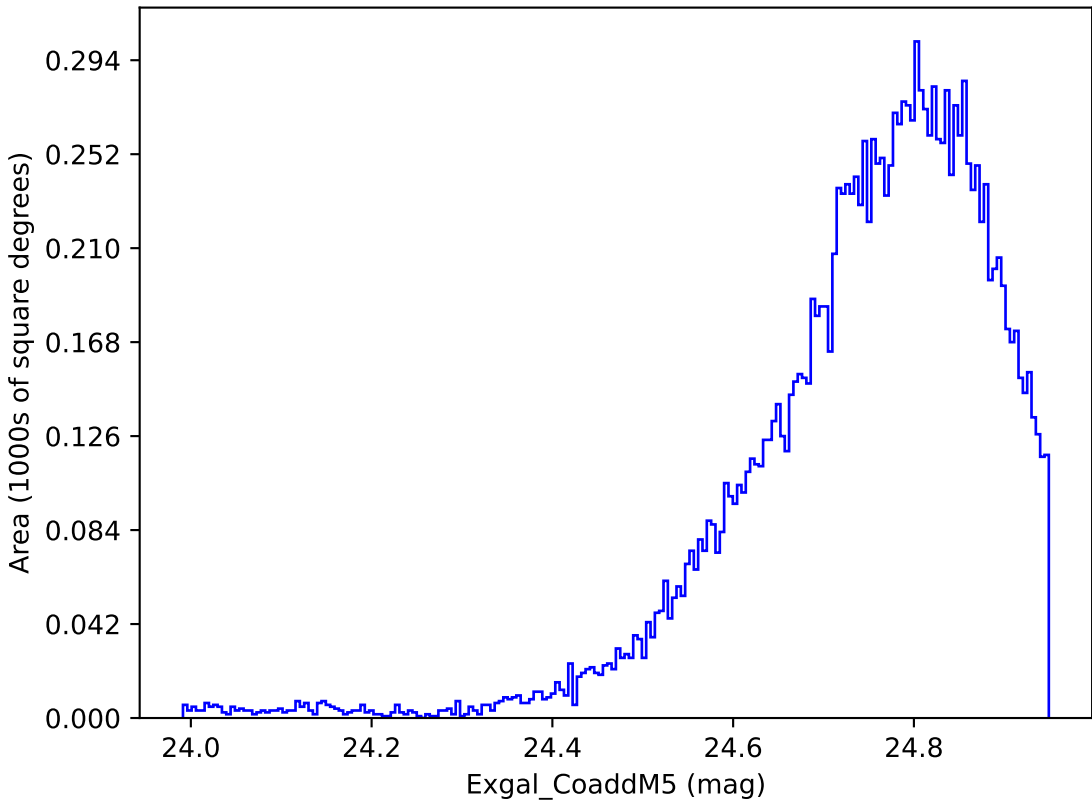
too_elab_r128_d2_gz_v3.4_10yrs WFD y band: Exgal_CoaddM5
