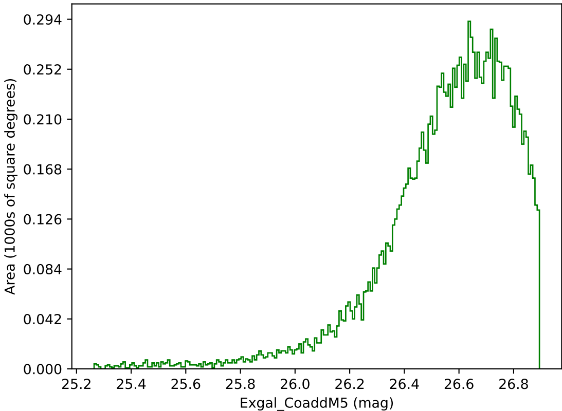
too_elab_r128_d2_gz_v3.4_10yrs WFD g band: Exgal_CoaddM5
