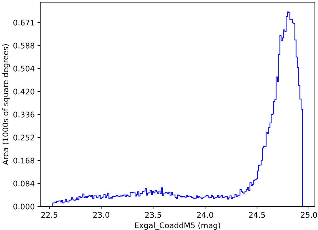
too_elab_r128_d2_gz_v3.4_10yrs All sky y band: Exgal_CoaddM5
