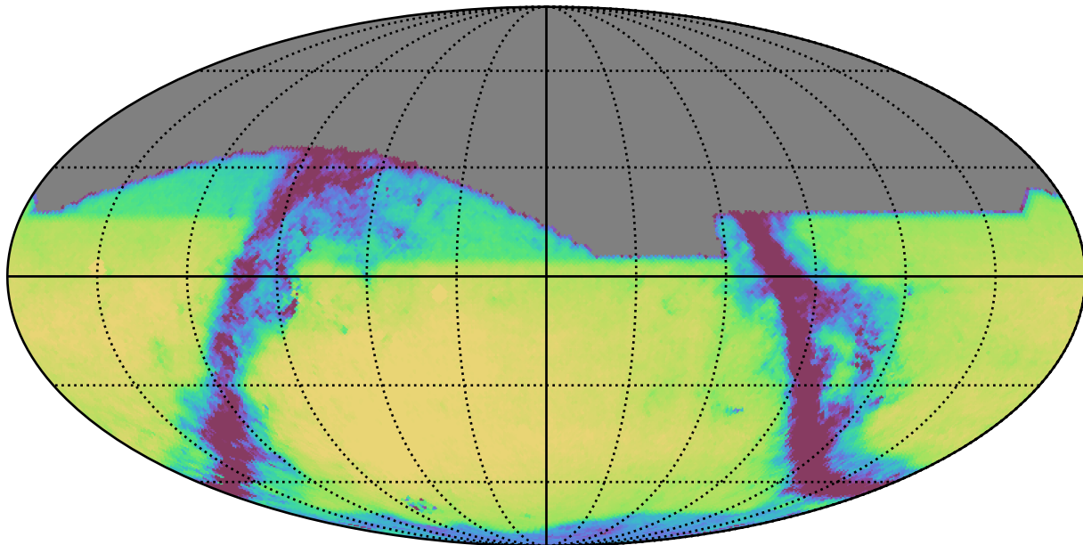
too_elab_r128_d2_gz_v3.4_10yrs All sky r band: Exgal_CoaddM5
