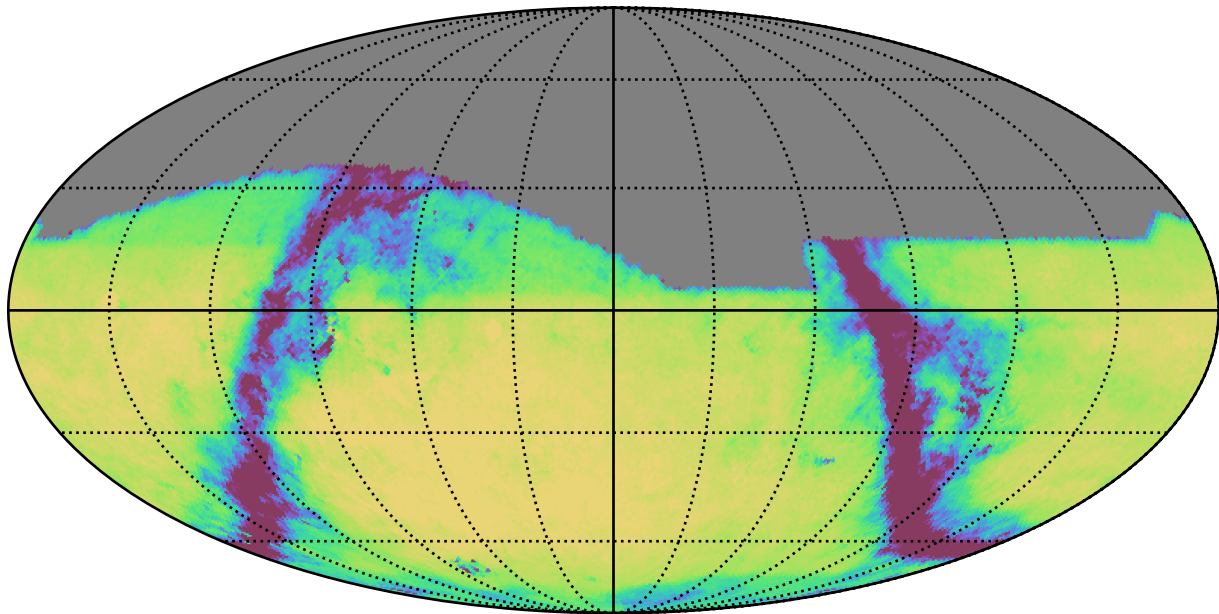
too_elab_r128_d2_gz_v3.4_10yrs All sky g band: Exgal_CoaddM5
