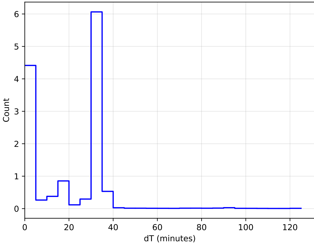
too_elab_r128_d2_gz_v3.4_10yrs All sky: DeltaT Histogram 1e6
