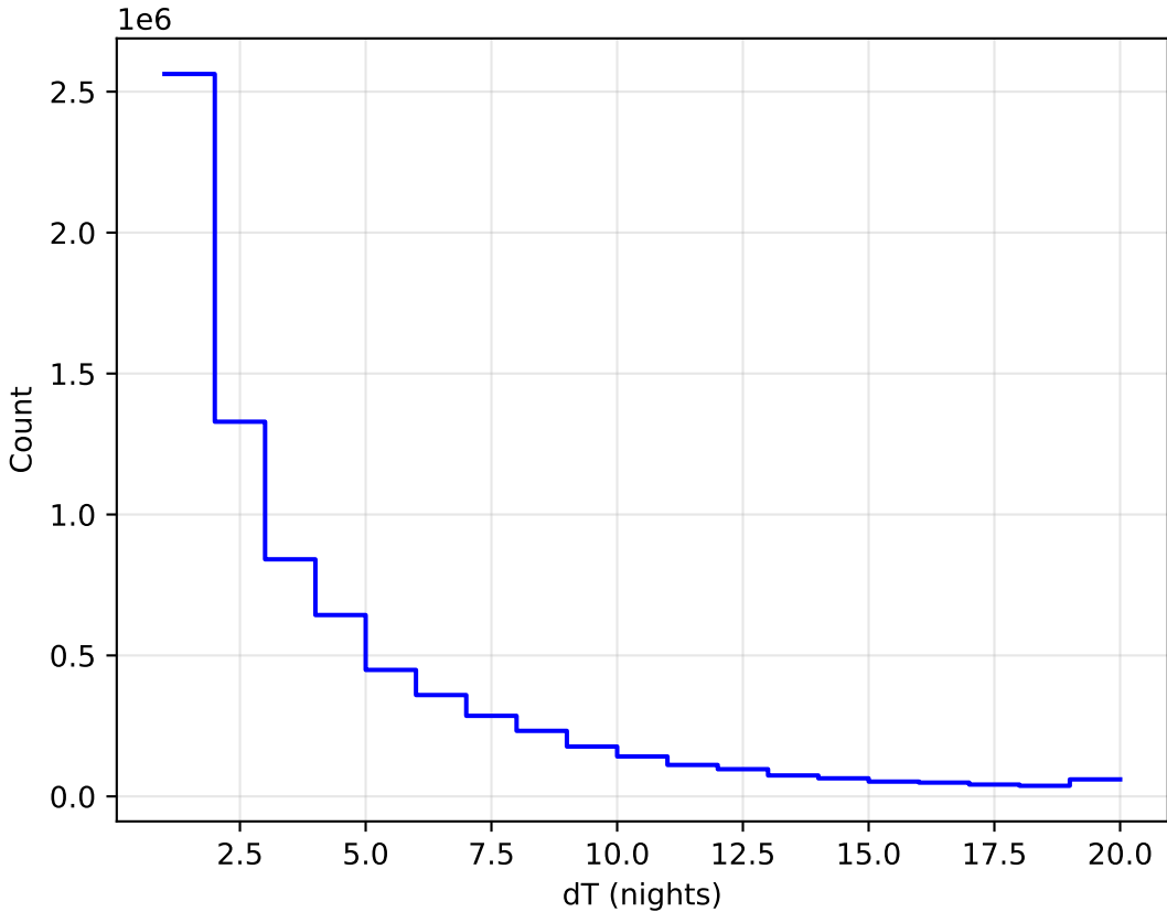
too_elab_r128_d2_gz_v3.4_10yrs WFD all bands: DeltaNight Histogram
