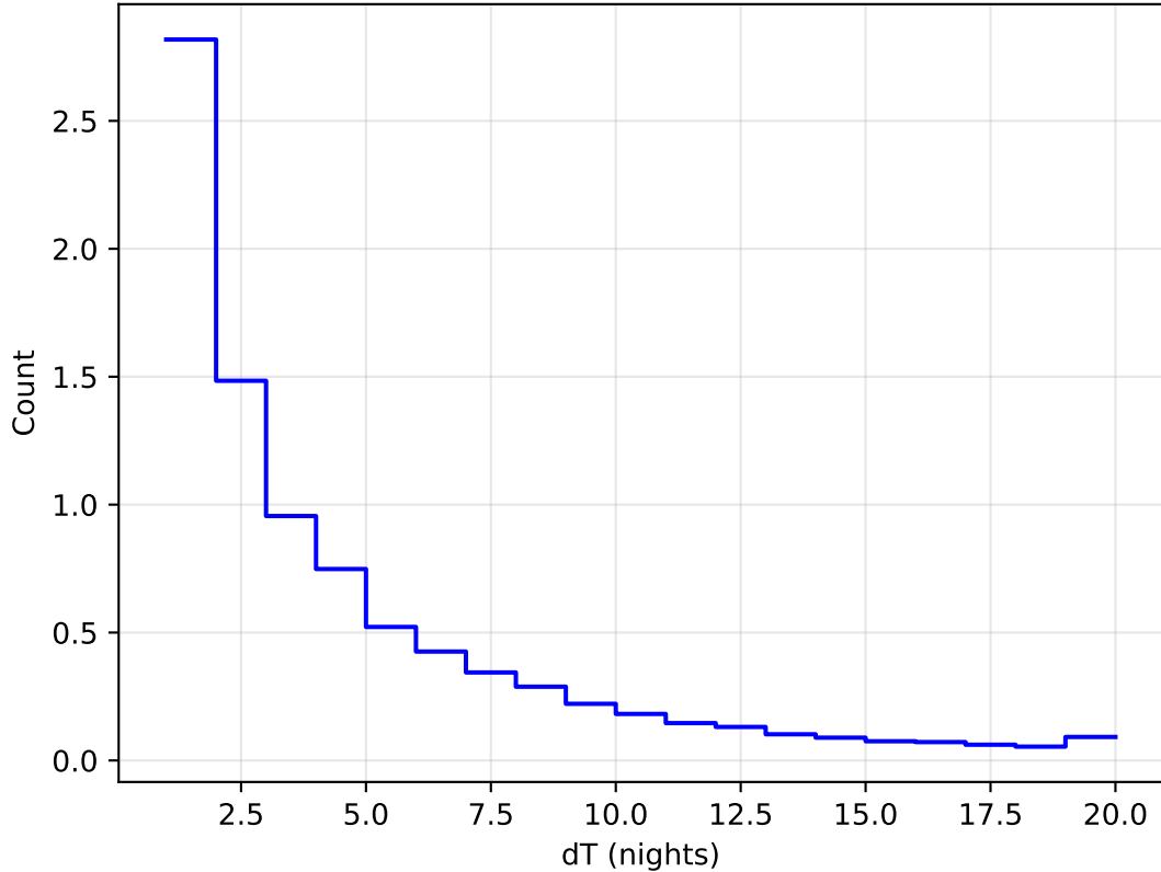
too_elab_r128_d2_gz_v3.4_10yrs All sky all bands: DeltaNight Histogram
