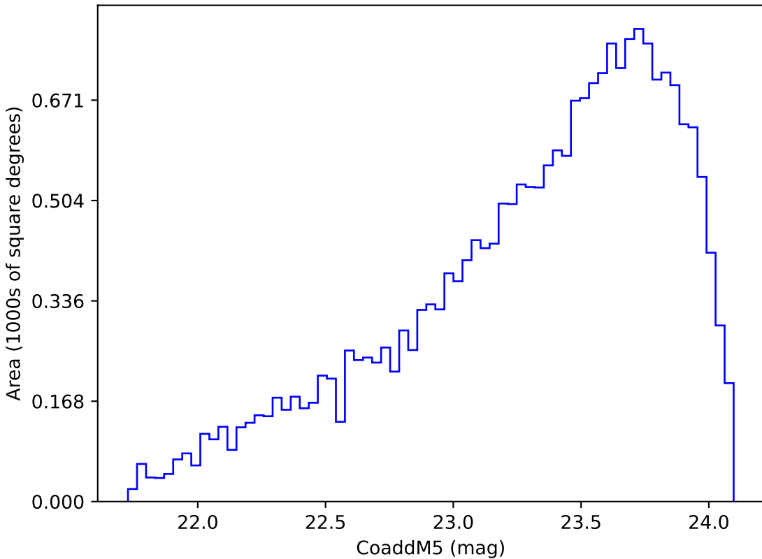
too_elab_r128_d2_gz_v3.4_10yrs Yr 3-4 y band: CoaddM5
