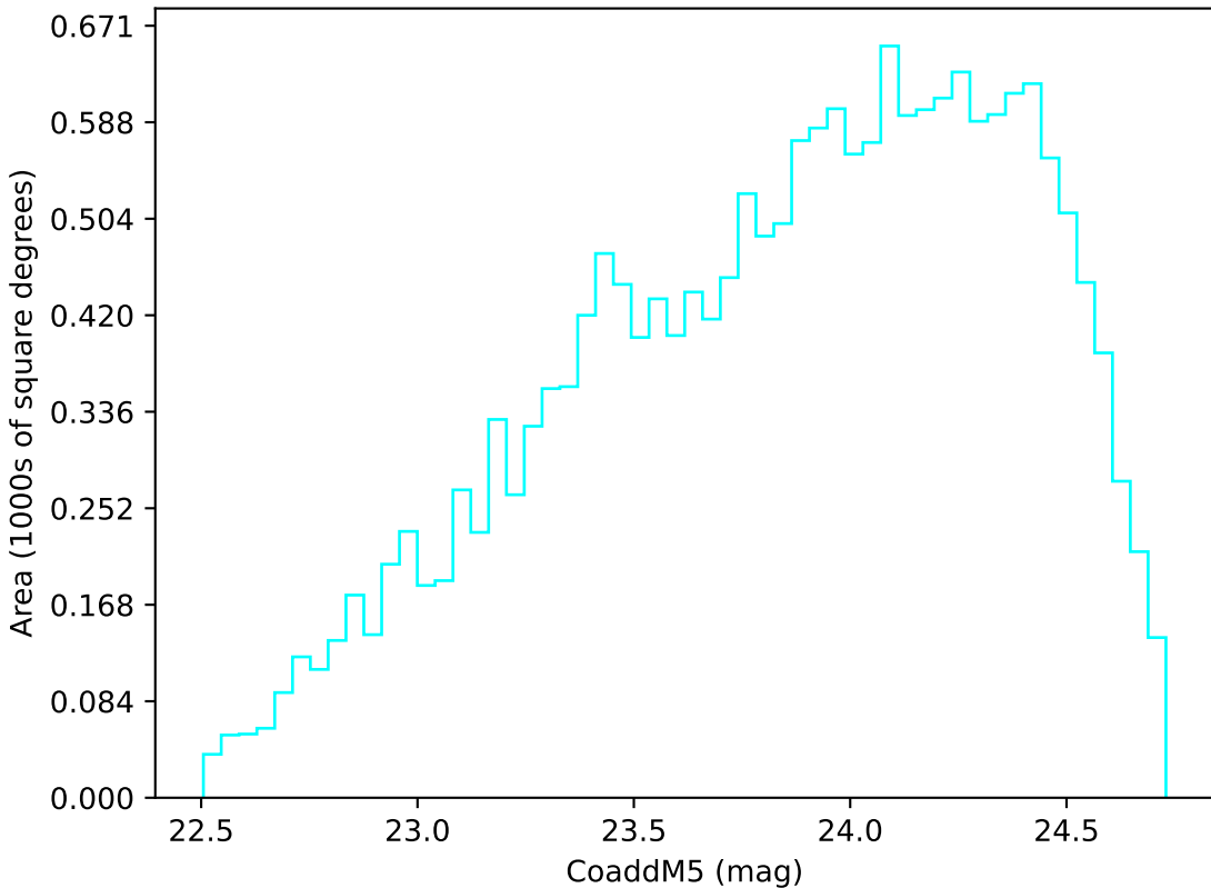
too_elab_r128_d2_gz_v3.4_10yrs Yr 3-4 u band: CoaddM5
