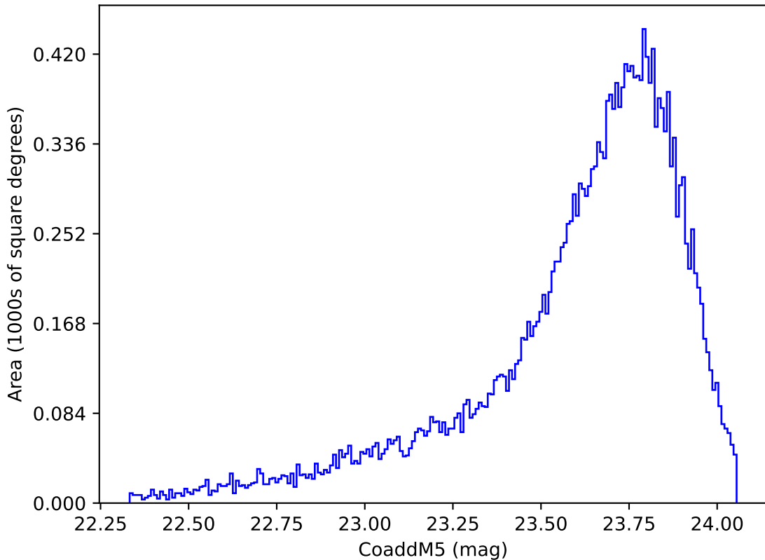
too_elab_r128_d2_gz_v3.4_10yrs Yr 1 y band: CoaddM5
