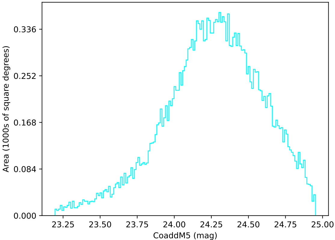
too_elab_r128_d2_gz_v3.4_10yrs Yr 1 u band: CoaddM5
