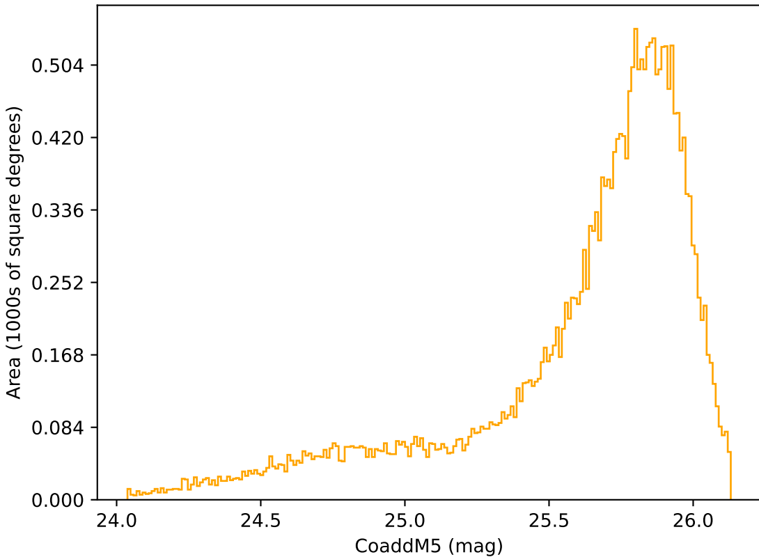
too_elab_r128_d2_gz_v3.4_10yrs Yr 1 r band: CoaddM5
