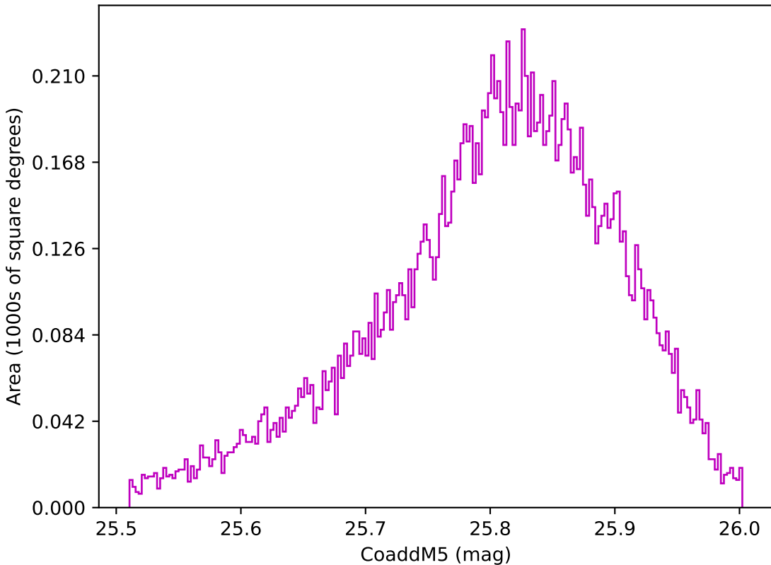
too_elab_r128_d2_gz_v3.4_10yrs WFD z band: CoaddM5
